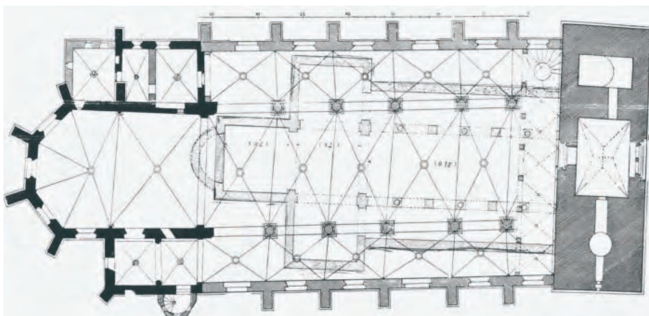
Fundamentplan
